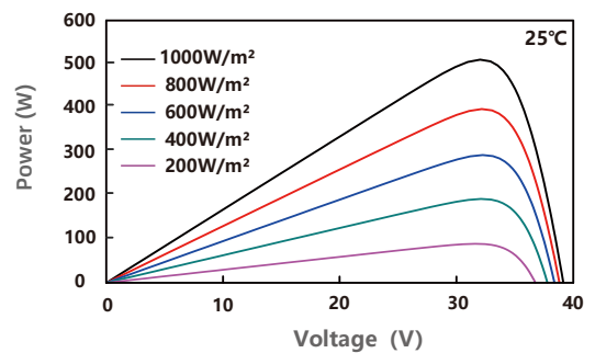
P-V Characteristics At Different Irradiations
